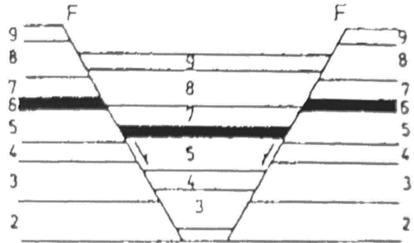
(a)地塹
