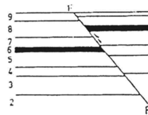
(c) 逆斷層 (Thrust Fault)
