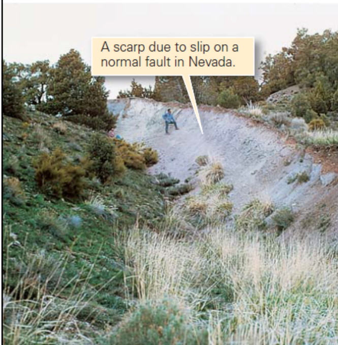
(a) A fault scarp develops where faulting displaces the land surface.
