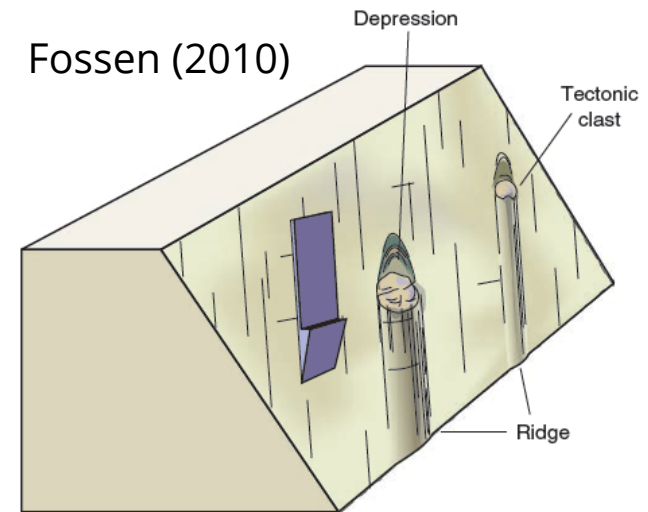
Figure 9.4 Pointed asperities or tectonic clasts sitting on fault surfaces may form depressions on the lee side and ridges on the opposite side. Such lineations are ridge-in-groove lineations.
