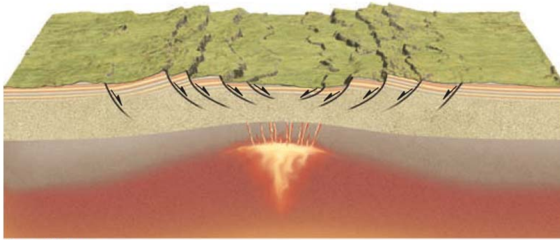
East Africa
